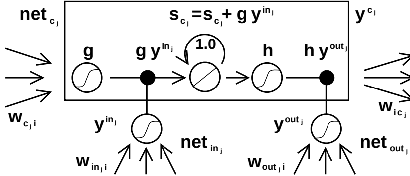
Figure 1: Architecture of memory cell c_j (the box) and its gate units in_j, out_j . The self-recurrent connection (with weight 1.0) indicates feedback with a delay of one time step. It builds the basis of the CEC. The gate units open and close access to CEC. See text and appendix A.1 for details.
